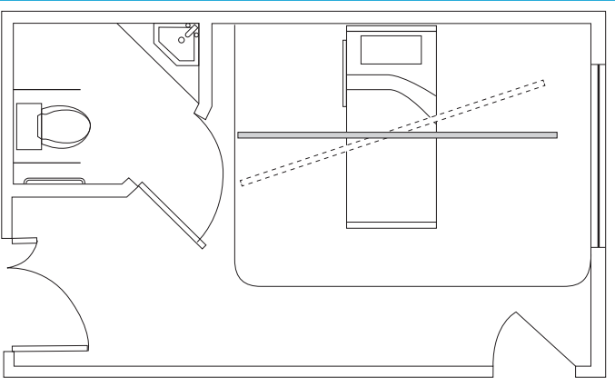
Straight Monorail – Bed To Chair
