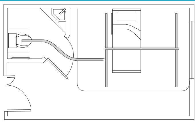
XY Gantry Ceiling Rail With access To Toilet
