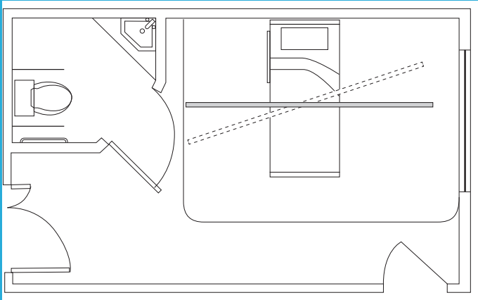
Straight Monorail – Bed To Chair
